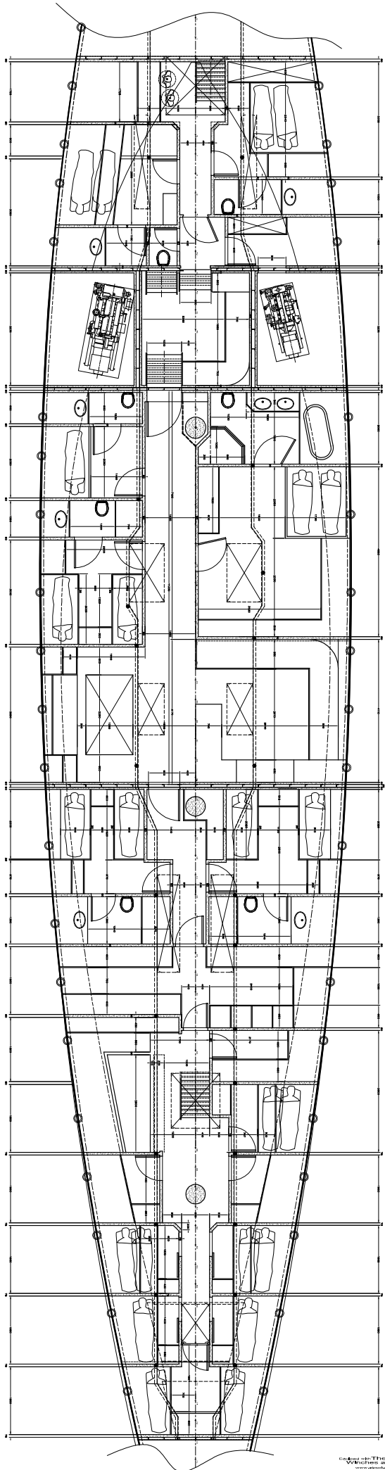
THE 3-MAST SCHOONER " ATLANTIC ", Designed by GARDNER & COX, 1903 Revised Accommodation Plan by Ed Kastelein Dated - 19.11.2008
